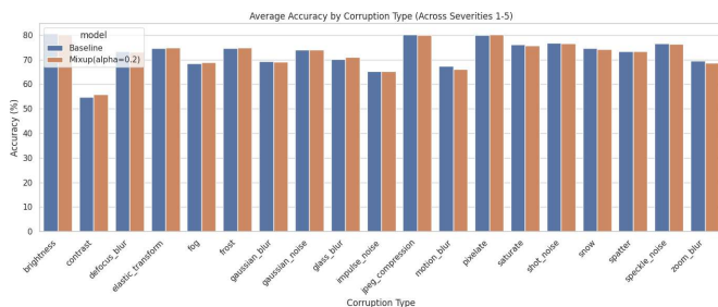
Fig. 1. Average CIFAR-10-C accuracy by corruption type for baseline and Mixup ( \alpha = 0.2 ) models.
